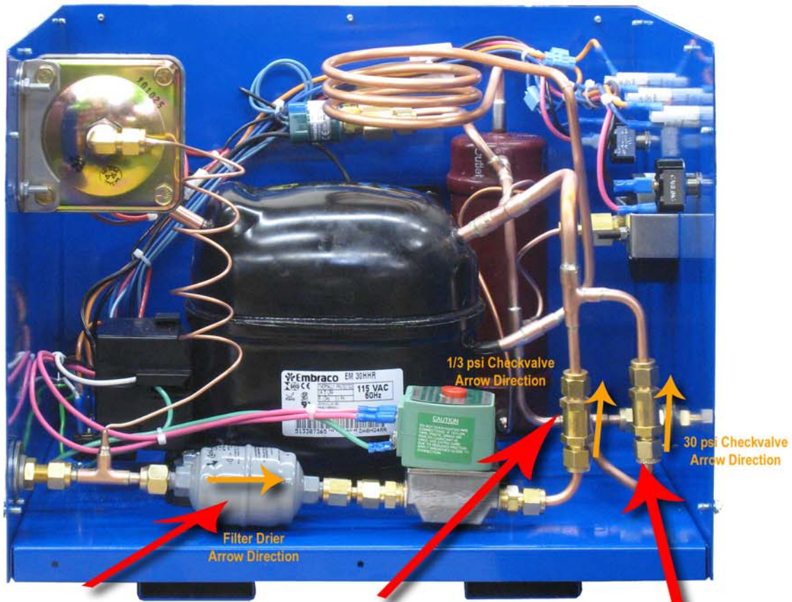
Filter Drier
